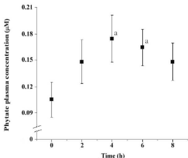
Figure 6. Phytate plasma concentration after ingestion of a single dose of 1400 mg dodecasodium phytate (1515 \mu\text{mol} of \text{InsP}_6 ) in humans; (a) significantly different from phytate concentration at time 0 h ( p < 0.05 ) (with permission from IOS Press BV, Amsterdam, NL [195]).
