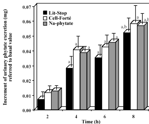
Figure 7. Urinary phytate excretion in humans 2–8 h after application of three different phytate supplements: 400 mg Lit-Stop (Ca-Mg-Phytate, 467 \mu\text{mol InsP}_6 ), 3200 mg Cell-Forté' (Ca-Mg-Phytate, 3734 \mu\text{mol InsP}_6 ) and 1400 mg Na-phytate (1515 \mu\text{mol InsP}_6 ) (a) vs. 2 h ( p < 0.05 ); (b) vs. 4 h ( p < 0.05 ). (with permission from IOS Press BV, Amsterdam, NL [195]).
